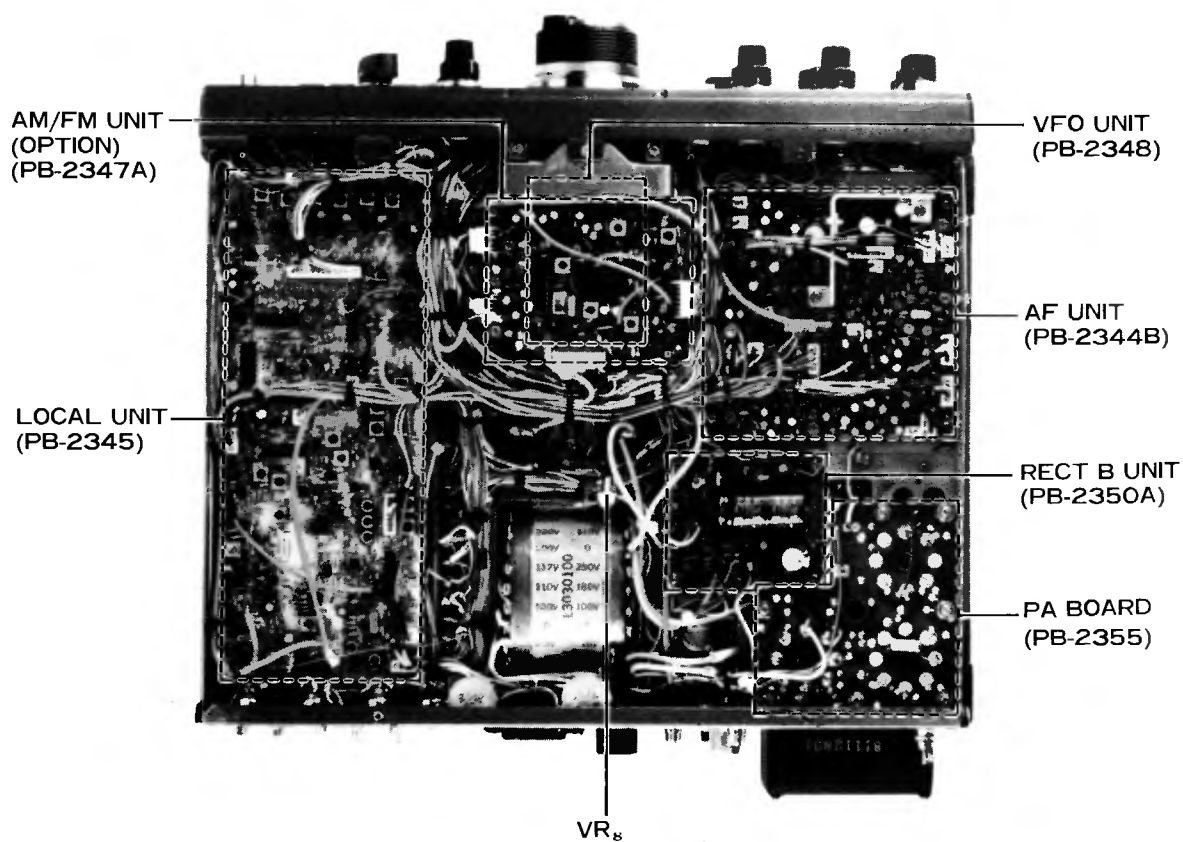
BOTTOM VIEW
