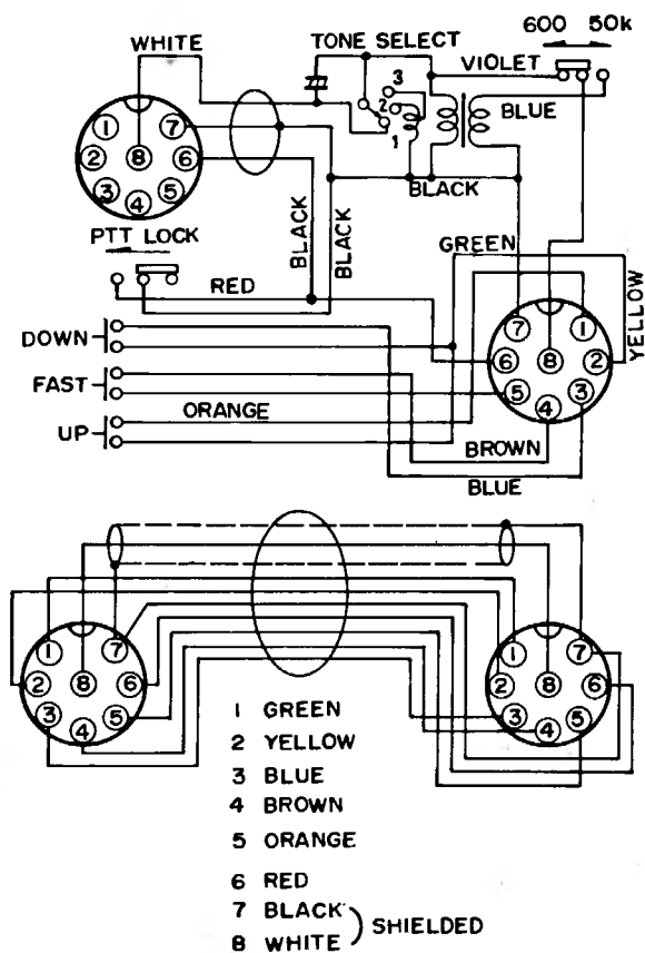
MD-1B8 MICROPHONE CONNECTIONS
